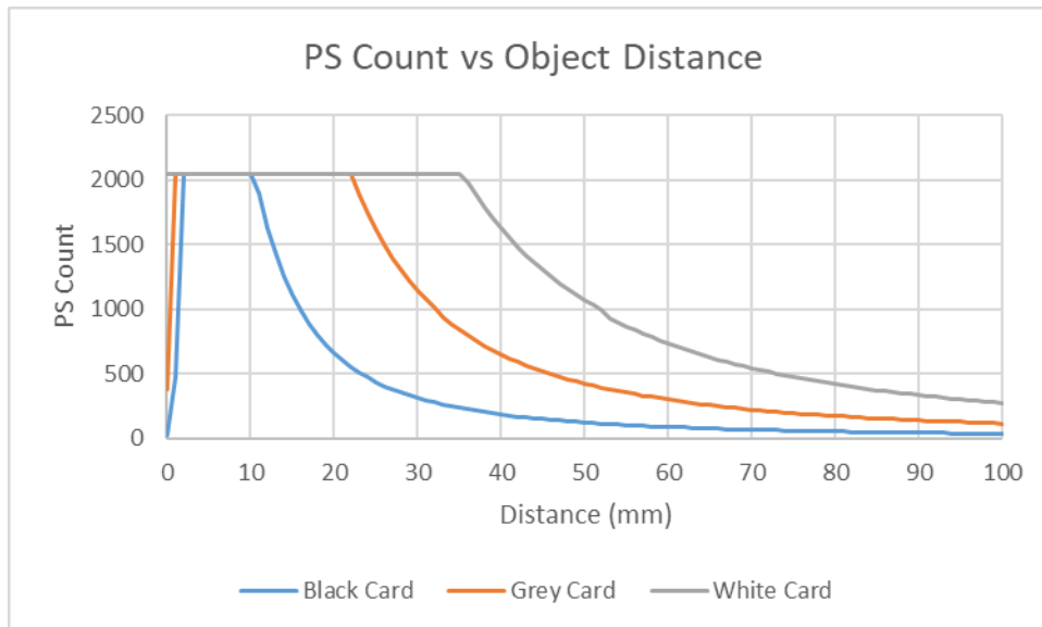
Figure 4.2: PS performance across distance 100mA, 32 pulse, 32us PW, 4x Averaging, Open Air (NO TP).
